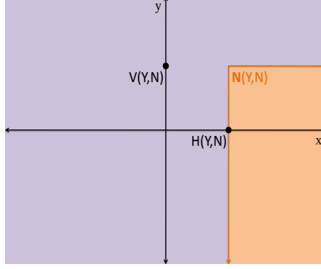
FIGURE 2. Cohesive Nash equilibria domain \mathbf{N}(Y, N) , (Mousa et al., 2014a).
