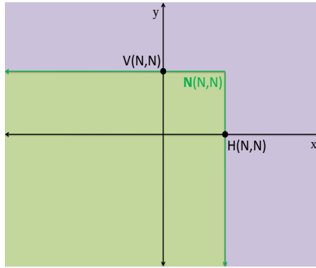
FIGURE 4. Cohesive Nash equilibria domain \mathbf{N}(N, N) , (Mousa et al., 2014a).
