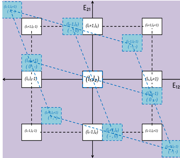
FIGURE 15. Rotating the pure strategies when the signs of (E_{12}, E_{21}) is (-, -) . The new order of the pure strategies moves to the small blue rectangles.
