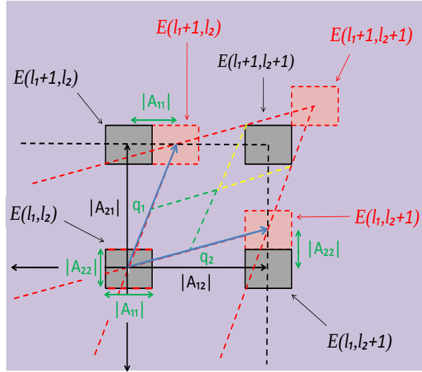
FIGURE 16. (l_1 + p, l_2 + q) is the mixed strategy when (E_{12}, E_{21}) is (+, +) .
