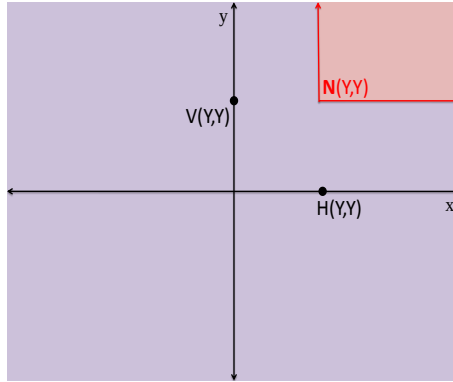
FIGURE 1. Cohesive Nash equilibria domain \mathbf{N}(Y, Y) , (Mousa et al., 2014a)
