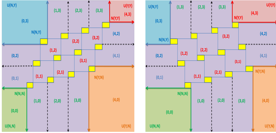
FIGURE 5. Disparate Nash equilibria when n_1 = 4 and n_2 = 3 . Left : A_{11} < 0 , A_{12} < 0 , A_{21} < 0 and A_{22} < 0 . The yellow rectangles include two pure Nash equilibria and a mixed Nash equilibria. Right : A_{11} < 0 , A_{12} > 0 , A_{21} < 0 and A_{22} < 0 . The yellow rectangles have no pure Nash equilibrium but include a mixed Nash equilibrium.
