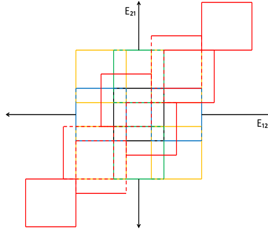
FIGURE 17. The bifurcations between the pure strategies when (E_{12}, E_{21}) = (+, +) .
