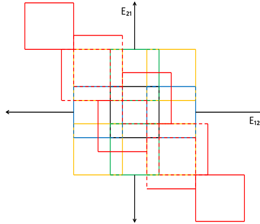
FIGURE 18. the bifurcations between the pure strategies when (E_{12}, E_{21}) = (-, -) .
