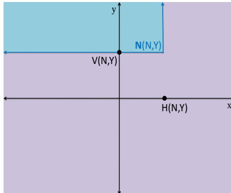
FIGURE 3. Cohesive Nash equilibria domain \mathbf{N}(N, Y) , (Mousa et al., 2014a).
